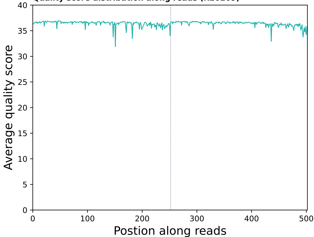
Quality score distribution along reads (R20209)
